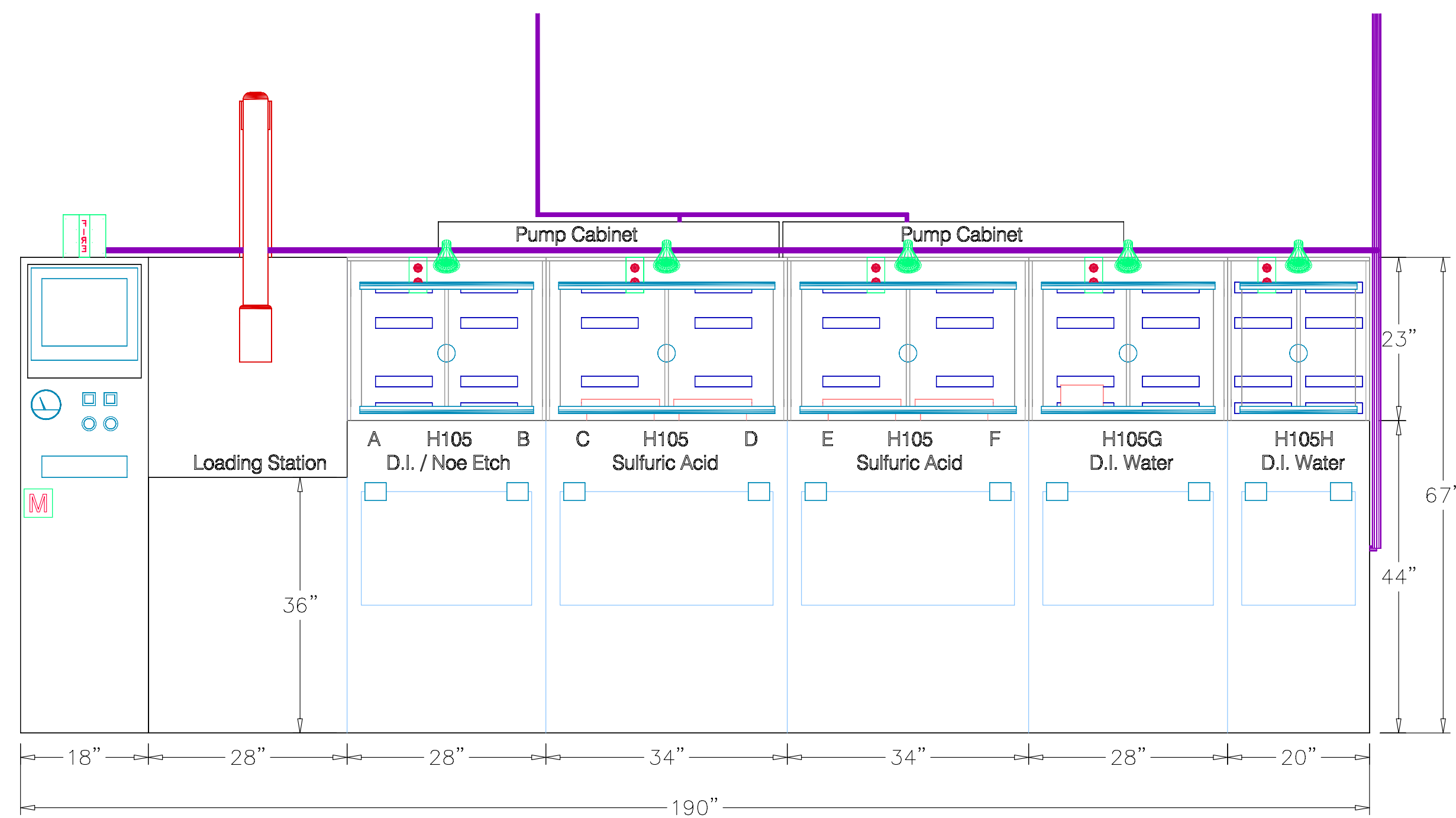
FRONT VIEW 3/4 inch = 1 Foot
